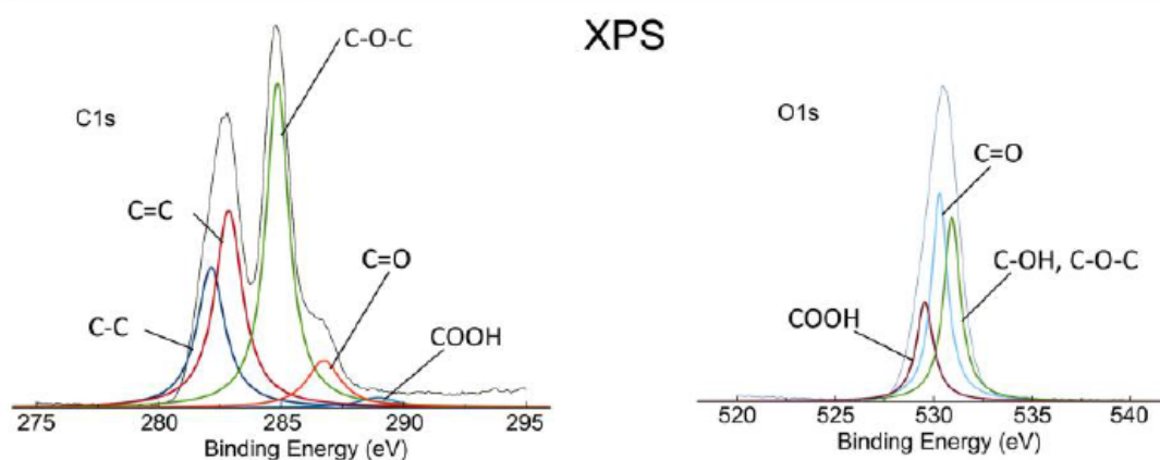
Fig.1 XPS spectra of oxidized carbon nanoparticles; C1s (left) and O1s (right)
